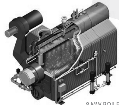
8 MW BOILER
